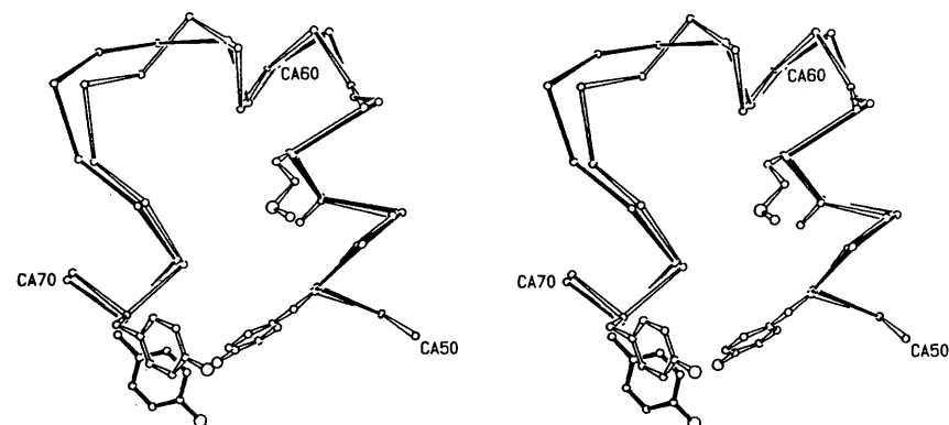
FIGURE 5: Stereoview showing the helix containing the site of mutation and the adjacent loop in WT (solid bonds) and K56M (open bonds). Notice that the backbone of helix and the loop in K56M moved closer compared to WT and that the side chain of Tyr-69 moved substantially. The side chains of the new hydrophobic triplet (Tyr-52, Ala-55, and Met-56) are shown for K56M.
