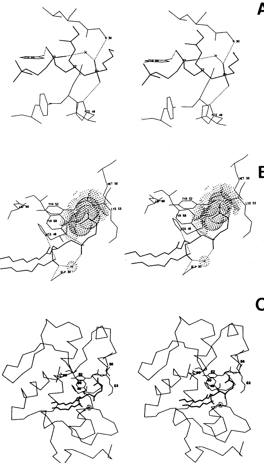
FIGURE 6: Stereoview of the K56M–DC 6 PC (tetrahedral analogue) complex obtained by docking the substrate into the enzyme active site according to the interactions indicated by White et al. (1990). The molecular modeling was carried out on an Evans and Sutherland PS330 using FRODO and the geometrical parameters of the substrate were optimized using X-PLOR. Panel A shows the interaction of the inhibitor with the active site residues in a view similar to that of Figure 3 in White et al. (1990). Panel B features the van der Waals interactions (dotted surfaces) between the trimethyl groups of choline and the hydrophobic pocket formed by Met-56, Tyr-52, and Tyr-69. Panel C shows the \alpha -carbon trace and side chains of a few active site residues of the entire complex. The heavy lines represent the structure of the lipid analogue.
