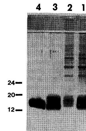
FIGURE 1: SDS-PAGE analysis of protein samples at different stages of the purification of WT PLA2: lane 1, insoluble inclusion pellet, before refolding; lane 2, insoluble pellet after refolding; lane 3, soluble fraction after refolding; lane 4, purified and activated PLA2. The additional strong band in lanes 1 and 3 is due to the pre-pro-PLA2.
