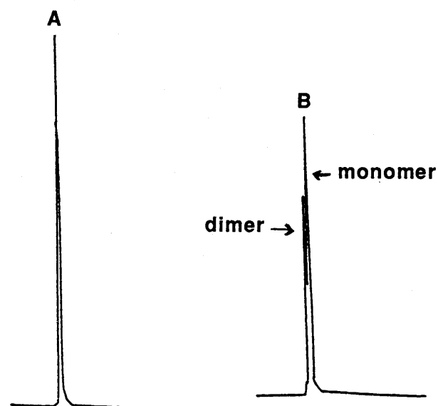
FIGURE 8: Fast flow Sepharose-12 gel filtration chromatography: (A) mixture of WT (monomeric) and K56M bovine PLA2; (B) mixture of C. atrox venom PLA2 (dimeric) and K56M bovine PLA2.
